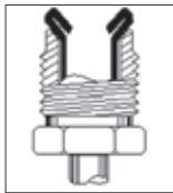
Flare tubing SAE (double) 7/16" - 24 thread
