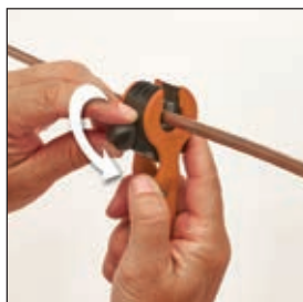
Spring-loaded automatic cutter: touch blade to tubing, turn dial 8 times, cut tubing
