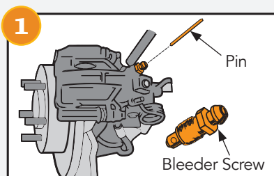
Insert Pin Into Bleeder Screw
