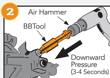
Install Removal Tool Into Air Hammer, Shock Bleeder From Top
